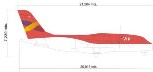
Drawing Title: Left Side Forward Page Number: 2 Original Issue Date: Junio 2005 Scale: 1:100 Aircraft Model: Domier 328
