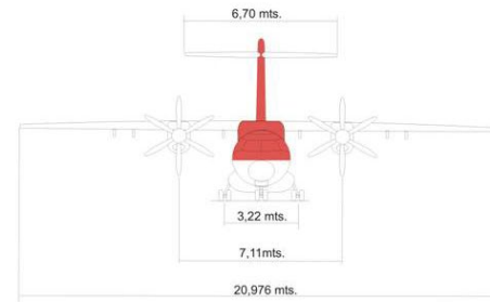
Drawing Title: Front View Page Number: 4 Original Issue Date: Junio 2005 Scale: 1:100 Aircraft Model: Domier 328
